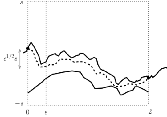
FIG 2. Illustration for the proof of the Fall event. The top and bottom solid black curves are h_t^{(1)}(\cdot) and h_t^{(2)}(\cdot) respectively. The event that h_t^{(1)}(y) - h_t^{(1)}(0) is less than -\epsilon^{1/2}s for some y \in (0, \epsilon) is \text{Fall}_{\epsilon, s} , and \mathbb{P}_{\mathbf{H}_t}^{1,2,(0,2),(h_t^{(1)}(0), h_t^{(1)}(2)), (+\infty, h_t^{(2)})}(\text{Fall}_{\epsilon, s}) is the probability of \text{Fall}_{\epsilon, s} conditioned on the sigma algebra \mathfrak{F}_{\text{ext}}(\{1\} \times (0, 2)) which is generated by everything outside of the first curve on the interval (0, 2) . The dashed black curve is a free Brownian bridge \tilde{B} with law \mathbb{P}_{\text{free}}^{(0,2),(h_t^{(1)}(0), h_t^{(2)}(2))} coupled to h_t^{(1)}(\cdot) so that it stays below h_t^{(1)}(\cdot) on the interval (0, 2) . Owing to this coupling, \mathbb{P}_{\mathbf{H}_t}^{1,2,(0,2),(h_t^{(1)}(0), h_t^{(1)}(2)), (+\infty, h_t^{(2)})}(\text{Fall}_{\epsilon, s}) \leq \mathbb{P}_{\text{free}}^{(0,2), h_t^{(1)}(0), h_t^{(1)}(2)}(\widetilde{\text{Fall}}_{\epsilon, s}) where \widetilde{\text{Fall}}_{\epsilon, s} is the Fall event with \tilde{B} in place of h_t^{(1)} . The probability of \widetilde{\text{Fall}}_{\epsilon, s} under \mathbb{P}_{\text{free}}^{(0,2), h_t^{(1)}(0), h_t^{(1)}(2)} conditioned on h_t^{(1)}(0) \leq s/4 and h_t^{(1)}(2) + 2 \geq -s/4 is maximized when h_t^{(1)}(0) = s/4 , and h_t^{(1)}(2) + 2 = -s/4 and the maximum value is equal to the probability of \inf_{z \in [0, \epsilon]} \{\tilde{B}(z) + z^2/2\} being less than -s\epsilon^{1/2} where \tilde{B} is a Brownian bridge in [0, 2] with \tilde{B}(0) = 0 and \tilde{B}(2) = -2 - 2^{-1}s . The reflection principle bounds this probability.
