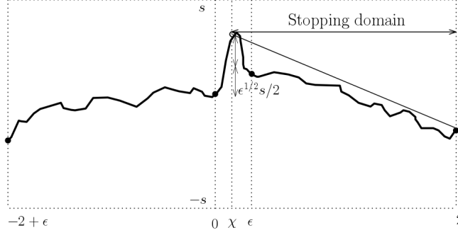
FIG 3. Illustration for the proof concerning the Rise event. The solid black curve is \mathfrak{h}_t^{(1)}(\cdot) . We start by rewriting the event \text{Rise}_{\epsilon,s} as \{\chi \leq \epsilon\} where \chi is the smallest x \in (0, \epsilon] such that \mathfrak{h}_t^{(1)}(x) - \mathfrak{h}_t^{(1)}(0) \geq \epsilon^{1/2}s ; if no such x satisfies this inequality, then \chi = +\infty . On the event \chi \leq \epsilon , the interval (\chi, 2) forms a stopping domain, thus by the strong Gibbs property the law of \mathfrak{h}_t^{(1)}(\cdot) on (\chi, 2) is that of a Brownian bridge conditioned to stay above \mathfrak{h}_t^{(2)} on that interval. We may couple \mathfrak{h}_t^{(1)}(\cdot) to lie above a free Brownian bridge. At any time in (\chi, 2) , a Brownian bridge has probability one-half of being above the linear interpolation between its endpoints (see the diagonal line in the figure). On the event \mathbf{G}_{\epsilon,s} , we can control the slope of such a linear interpolation by a constant c time s . Thus, between \chi and \epsilon , the linear interpolation may have dropped at most c\epsilon which, for \epsilon small enough is bounded by \epsilon^{1/2}s/2 . The means that, on the event that \chi \leq \epsilon , there is at least a one-half chance of \mathfrak{h}_t^{(1)}(\epsilon) - \mathfrak{h}_t^{(1)}(0) \geq \epsilon^{1/2}s/2 . However, viewed with a backwards' glance from position \epsilon , this occurrence is a Fall event; so that the just given argument concerning Fall yields a Gaussian tail for the probability of the event in question.
